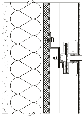
Horizontal Section
