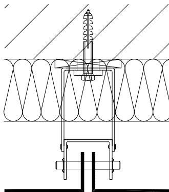
Horizontal Section
