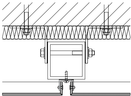
Horizontal Section
