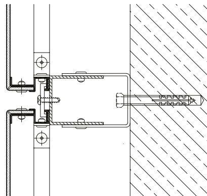
Vertical Section
