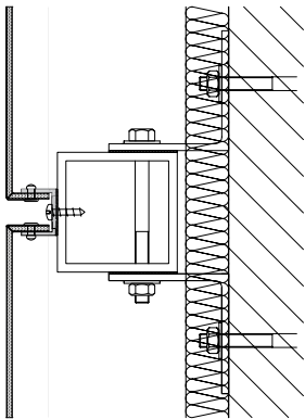
Vertical Section
