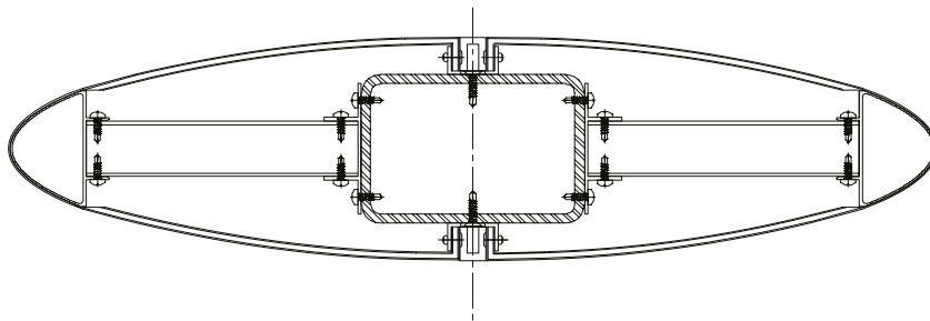
Section Drawing
