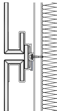
Vertical Section
