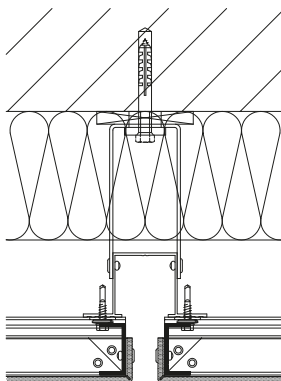
Horizontal Section
