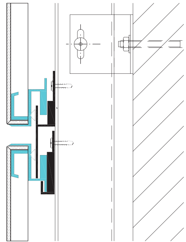
Vertical Section
