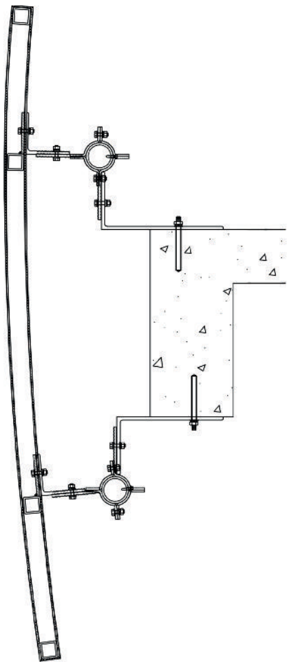
Vertical Section
