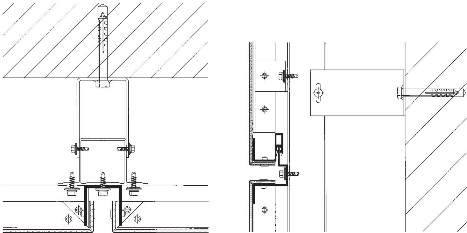
Horizontal Section
