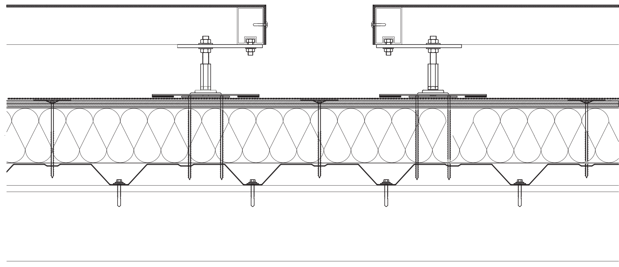
Vertical Section
