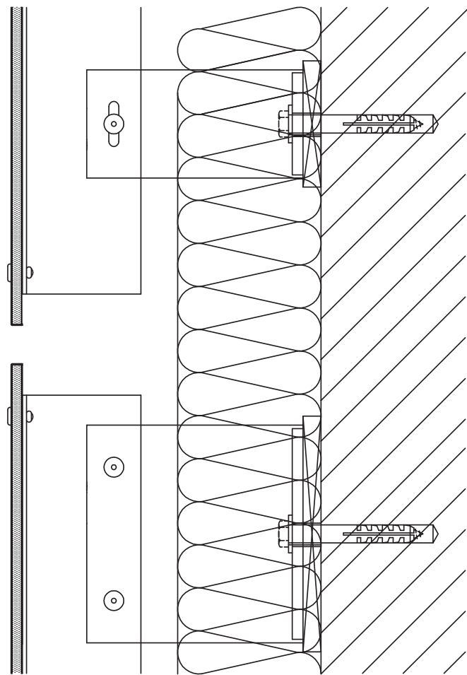
Vertical Section
