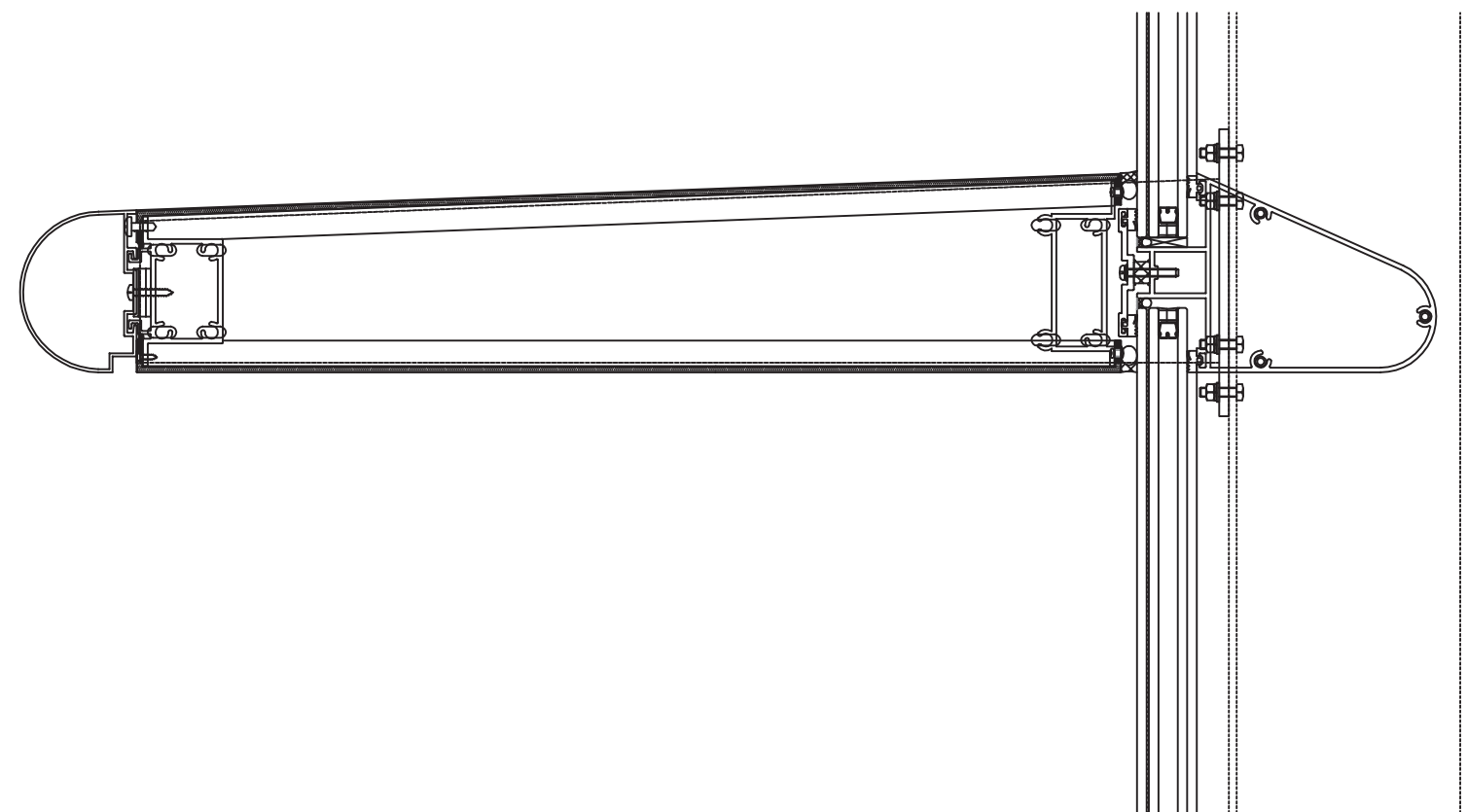
Vertical Section
